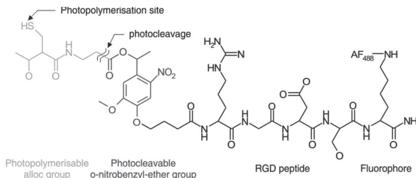
Scheme 2. RGD peptide (black) fluorescently labelled with the fluorophore Alexa Fluor 488 (AF 488 ) bound to photocleavable o-nitrobenzyl ether (dark grey) and photopolymerisable alloc groups (light grey); the molecule can be reversibly polymerized to a PEG based hydrogel via thiol-ene photoreaction. Adapted with permission. [102] Copyright 2012, Wiley-VCH.
