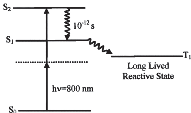
Scheme 1. Energy level diagram for two-photon excitation of rose bengal. Reproduced with permission. [75] Copyright 2000, American Chemical Society.
